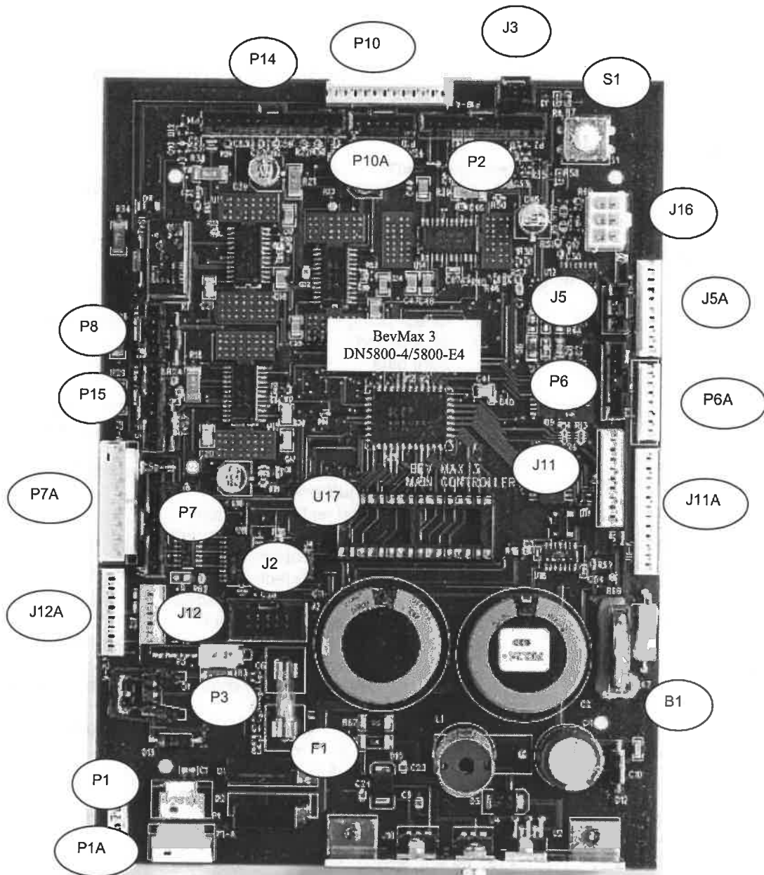
BEVMAX 3 5800-4 MDB CONTROLLER CONNECTIONS
