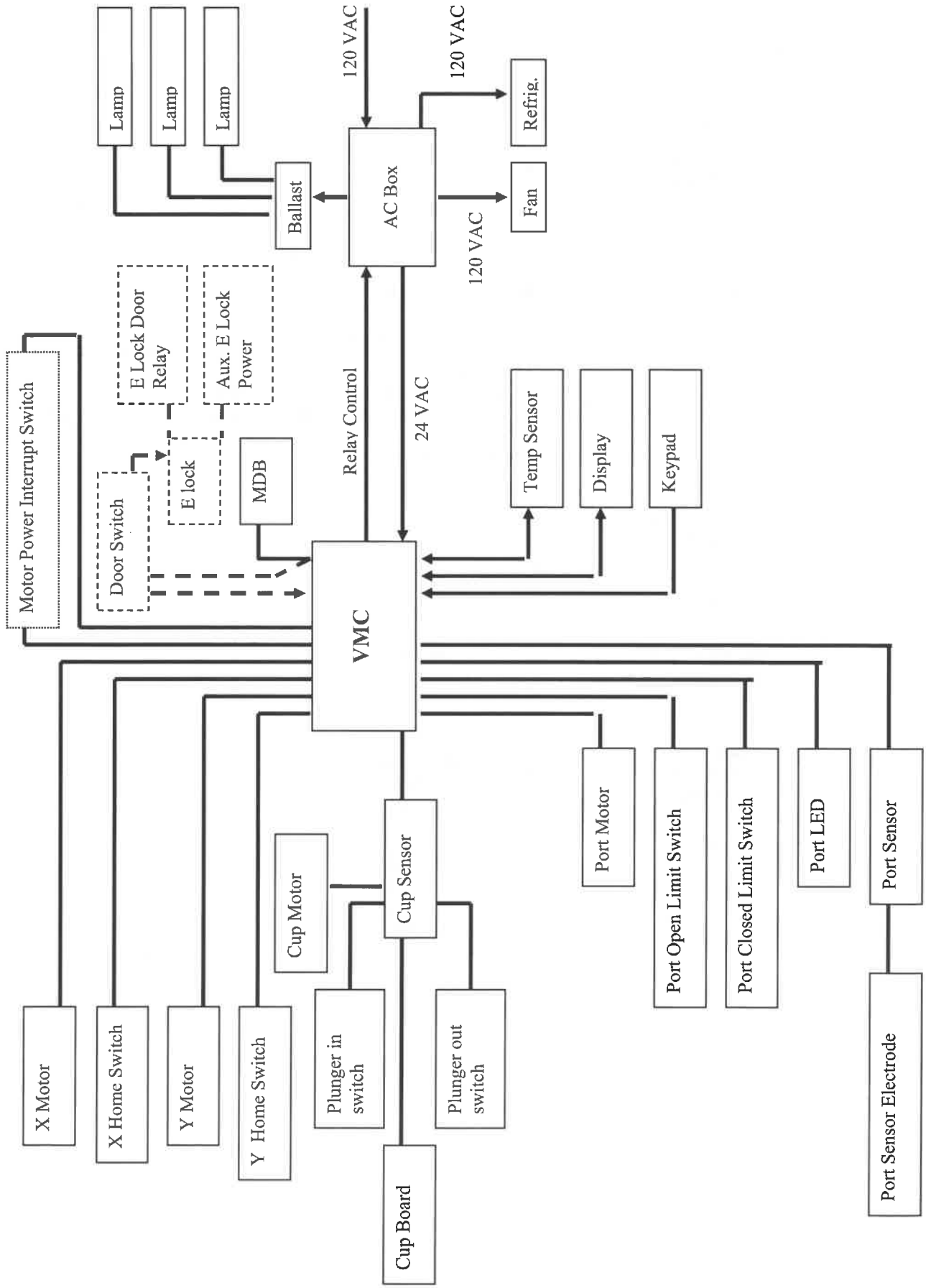
BevMax 3 5800-4 Domestic Block Diagram
